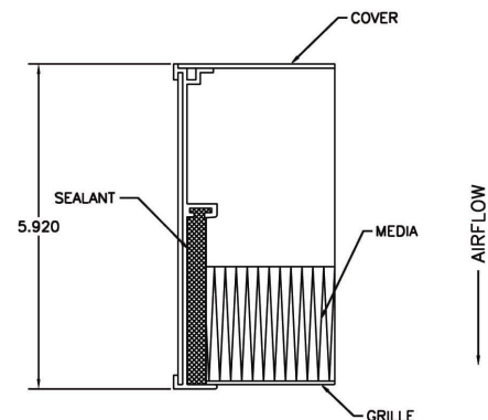
FRAME CROSS-SECTION
